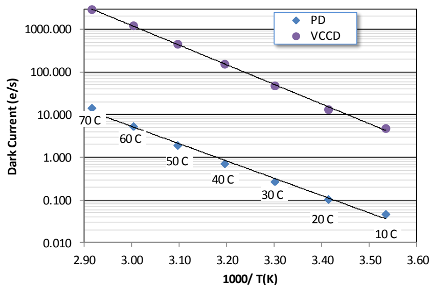
Figure 9: Dark Current versus Temperature
