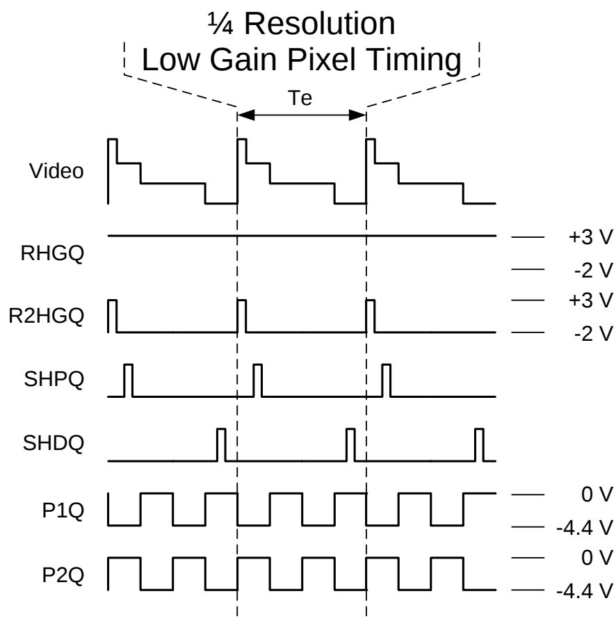
Figure 30: \frac{1}{4} resolution low gain pixel timing. See Table 4 center columns for pin assignments.
