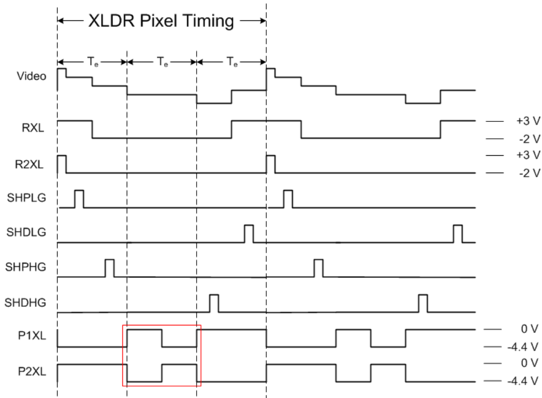
Figure 32: XDLR Timing with Variable HCCD clocking. See Table 4 right columns for pin assignments.
