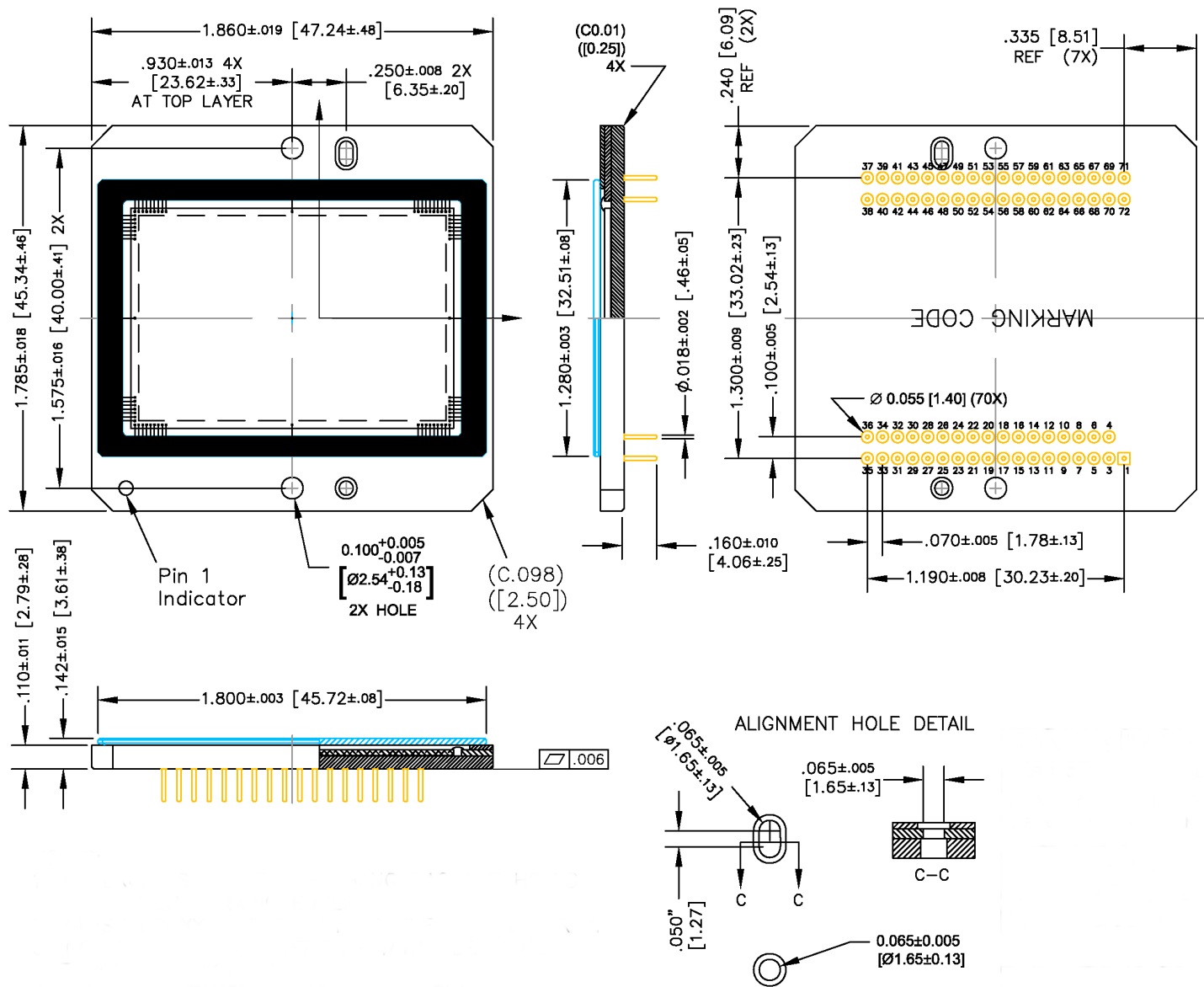
Figure 35: Completed Assembly (1 of 2)
