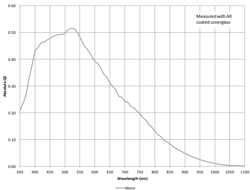
Figure 5: Monochrome with Microlens Quantum Efficiency
