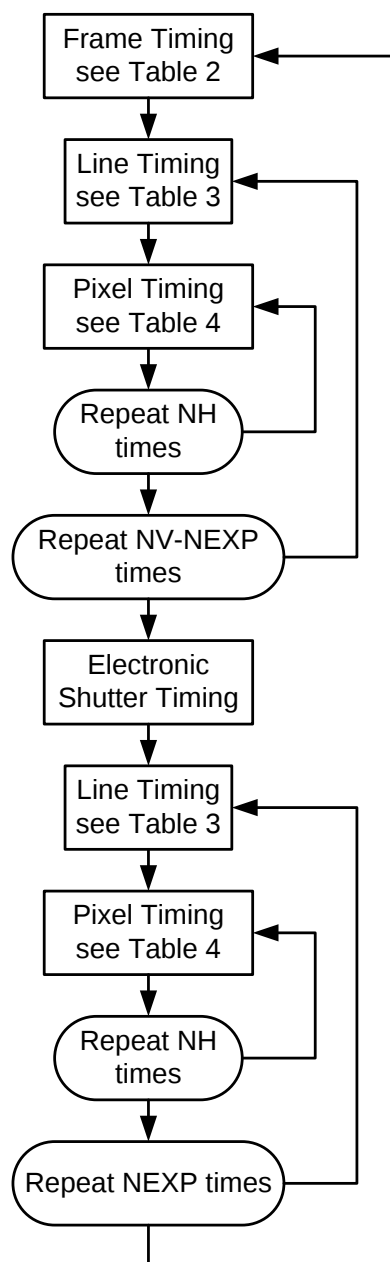
Figure 18: The timing flow chart using the electronic shutter for exposure control.
