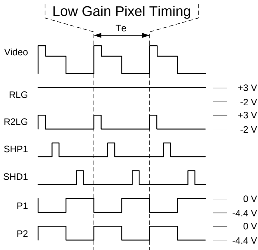
Figure 28: Low gain pixel timing. See Table 4 left columns for pin assignments.
