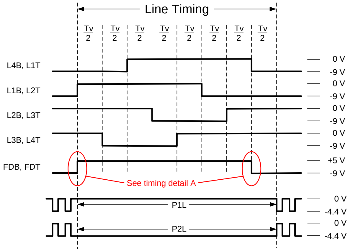
Figure 22: The line timing diagram. See Table 3 for device pin assignments
