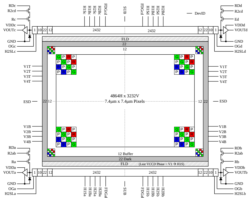
Figure 3: TRUESENSE Sparse Color Filter Pattern
