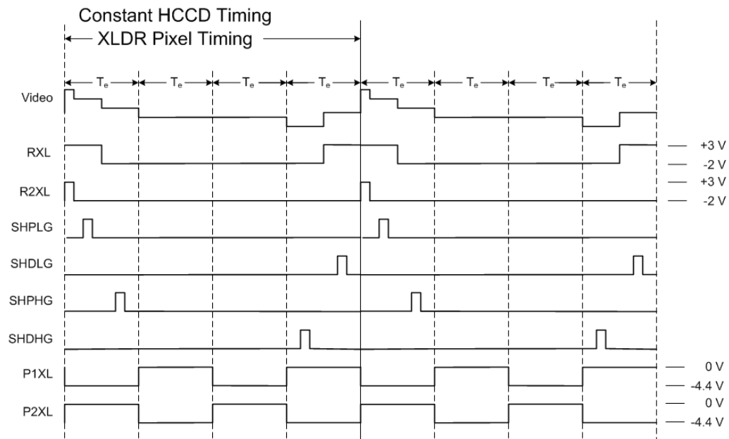
Figure 31: XDLR Timing with Constant HCCD. Operating at 20MHz. See Table 4 right columns for pin assignments.
