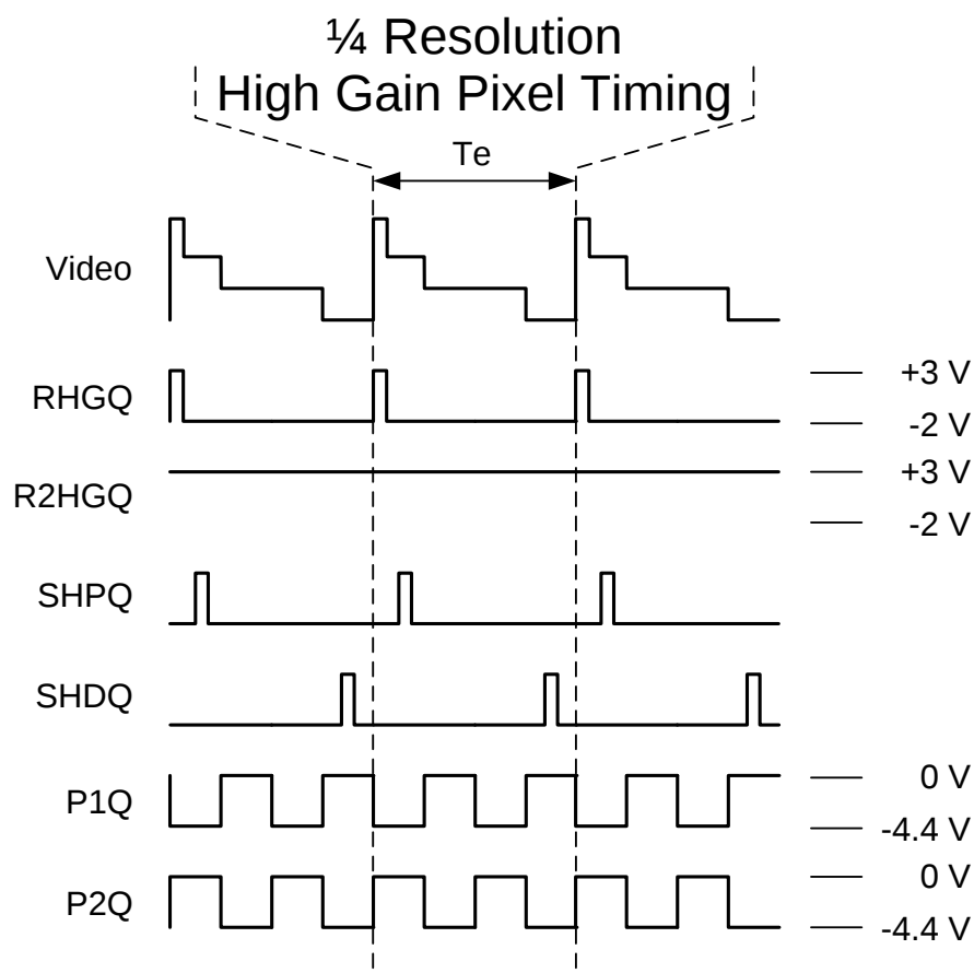
Figure 29: \frac{1}{4} resolution high gain pixel timing. See Table 4 center columns for pin assignments.
