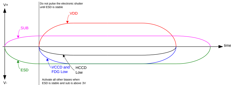
Figure 14: Power Up and Power Down Sequence
