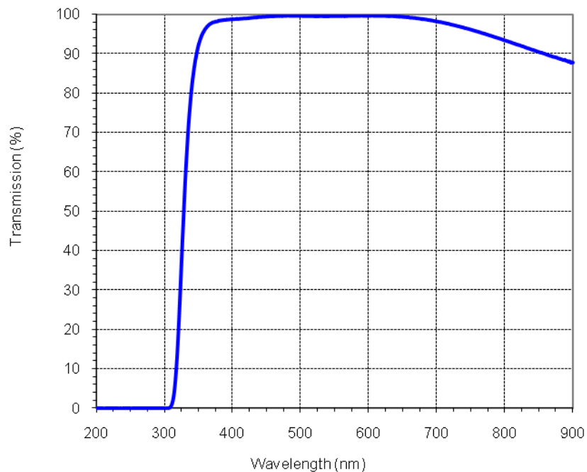
Figure 38: Cover Glass Transmission
