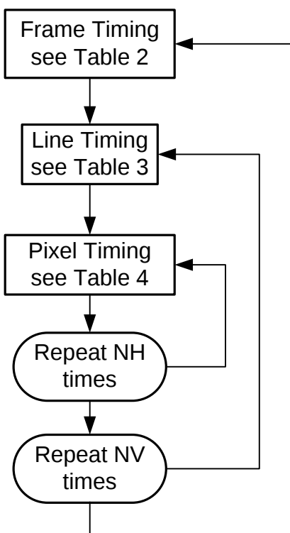
Figure 17: The timing flow when the electronic shutter is not used.
