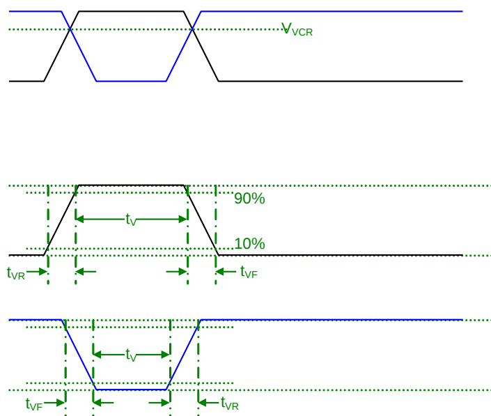
Figure 34: VCCD Clock Rise Time, Fall Time and Edge Alignment
