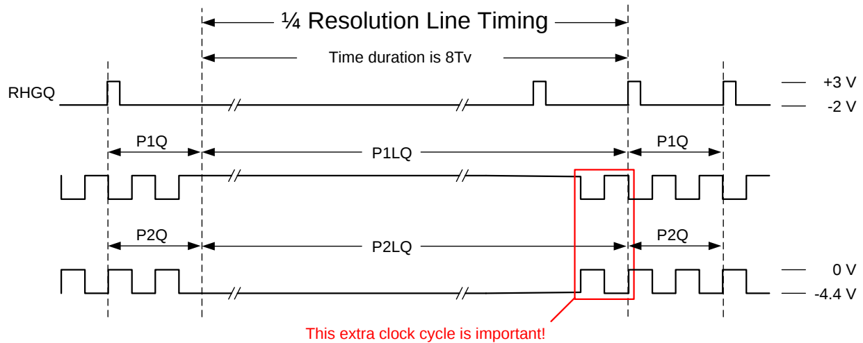
Figure 24: 1/4 resolution line timing diagram. See Table 3 center columns for pin assignments.
