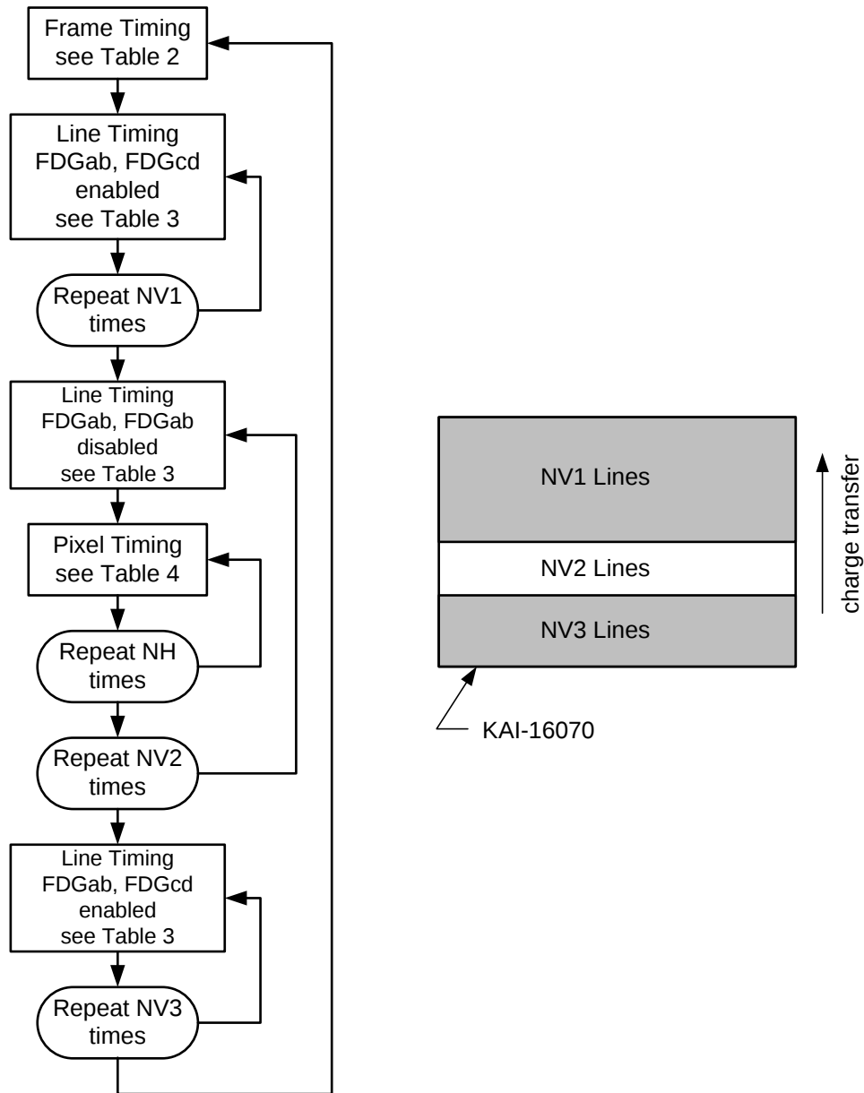
Figure 19: Sub window timing flow chart.
