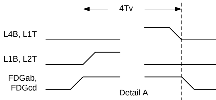
Figure 23: Fast dump gate timing detail A. See Table 3 for device pin assignments
