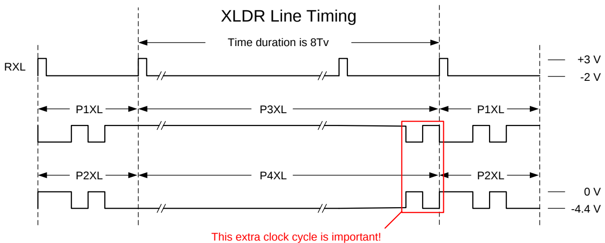
Figure 25: The XDLR line timing diagram. See Table 3 right columns for pin assignments.
