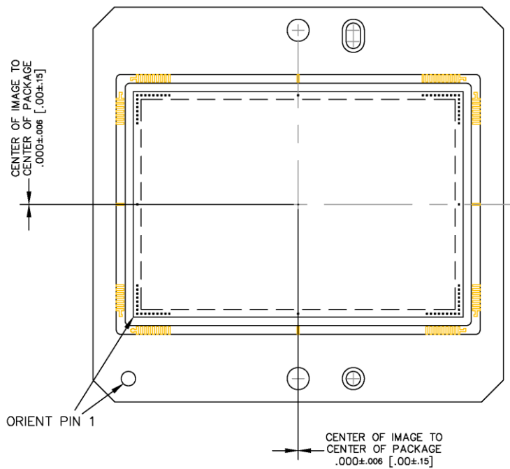
Figure 36: Completed Assembly (2 of 2)
