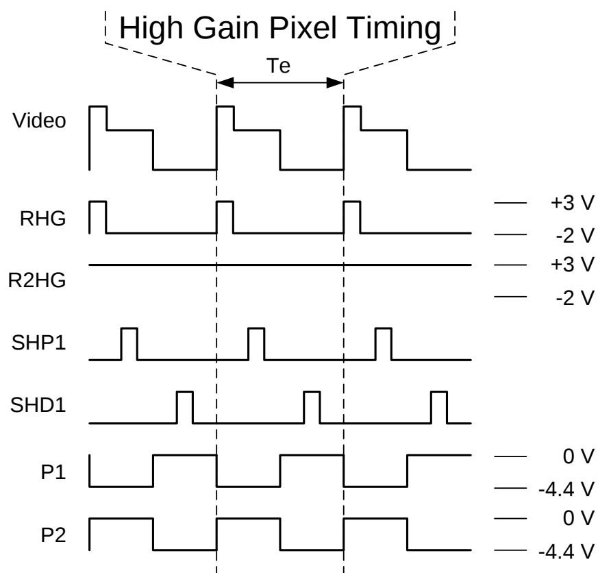
Figure 27: High gain pixel timing. See Table 4 left columns for pin assignments.
