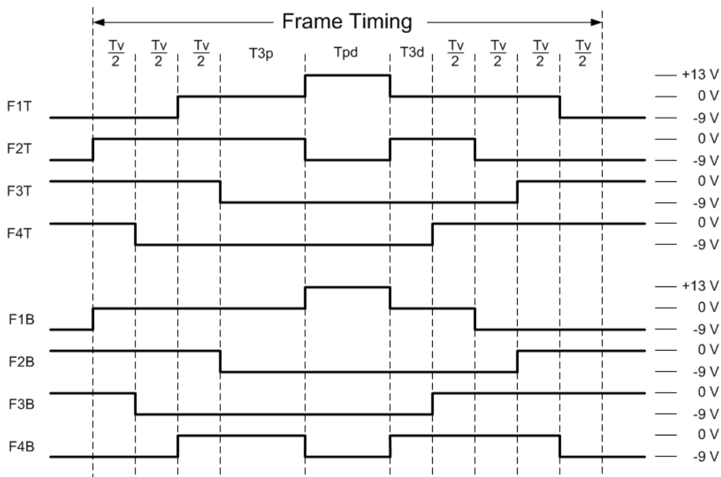
Figure 21: The frame timing diagram. See Table 2 for pin assignments
