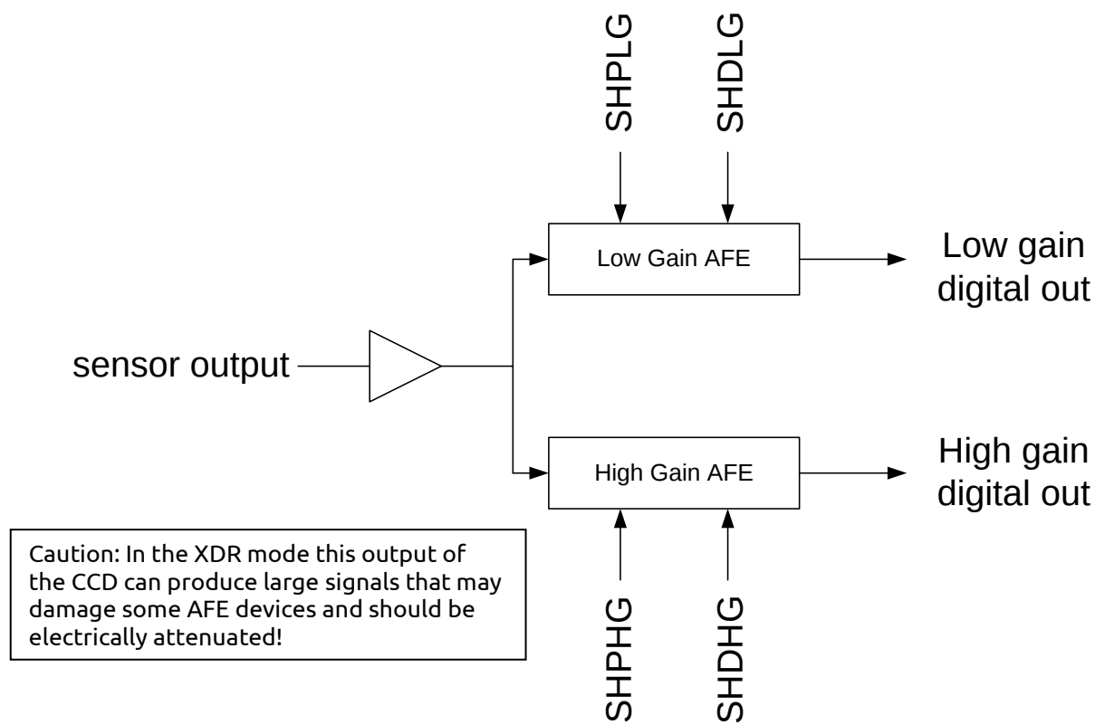
Figure 33: A block diagram showing the AFE connections for XLDR timing.
