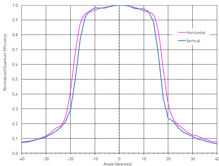
Figure 8: Monochrome with Microlens Angular Quantum Efficiency
