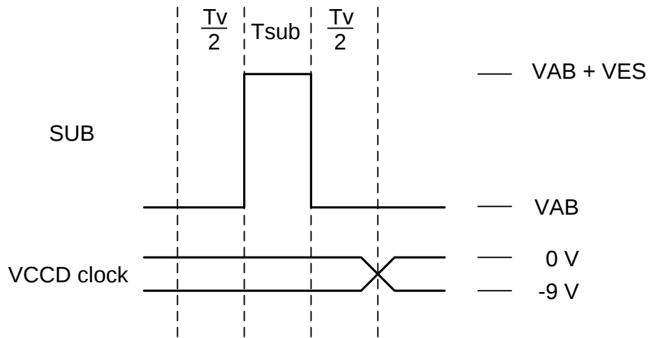
Figure 26: Electronic shutter timing diagram.
