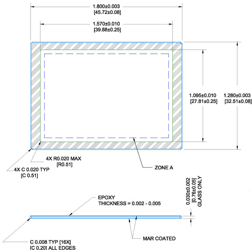
Figure 37: Cover Glass
