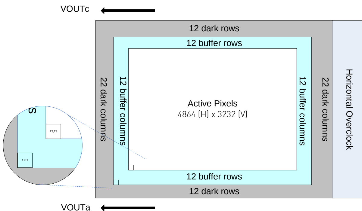
Figure 12: Regions of Interest
