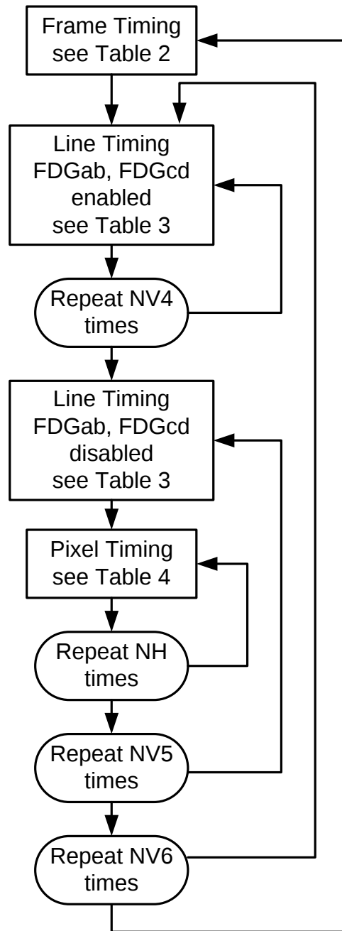
Figure 20: The timing flow chart to alternately skip and read rows for subsampling.
