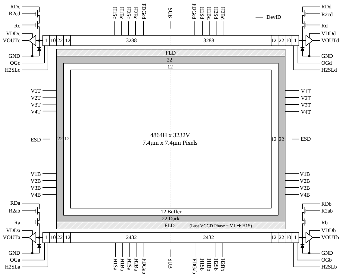
Figure 1: Block Diagram
