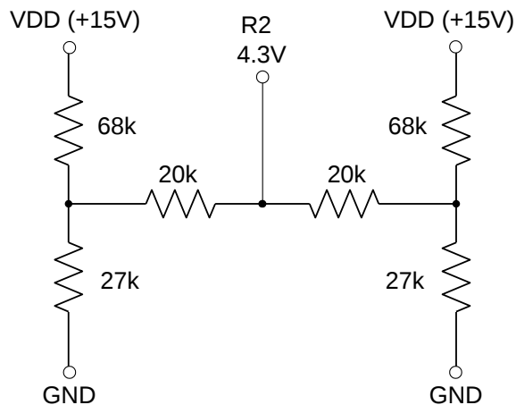
Figure 13: Equivalent Circuit for Reset Gate, low Gain (R2ab and R2cd)
